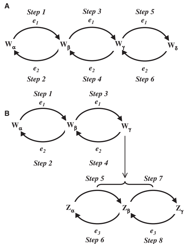
Fig. 8. (A) Diagram with four different protein W forms, W_\alpha, W_\beta, W_\gamma and W_\delta . The arrows show the interconversion between the forms: W_\alpha \rightarrow W_\beta (step 1); W_\beta \rightarrow W_\alpha (step 2); W_\beta \rightarrow W_\gamma (step 3); W_\gamma \rightarrow W_\beta (step 4); W_\gamma \rightarrow W_\delta (step 5); and W_\delta \rightarrow W_\gamma (step 6). Steps 1, 3 and 5 are catalyzed by the same enzyme ( e_1 ). The second, fourth and sixth steps are catalyzed by another enzyme ( e_2 ). (B) Network diagram with two interconvertible proteins W and Z. Each protein has three different forms, W_\alpha, W_\beta, W_\gamma , and Z_\alpha, Z_\beta, Z_\gamma , respectively. The modification and demodification steps of protein W are catalyzed by e_1 and e_2 , respectively. The modification steps of protein Z are catalyzed by the active form of the protein W ( W_\gamma ), and the demodification steps are catalyzed by the enzyme e_3 .
